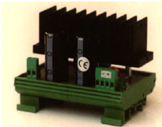
mod.: PLxx/6 L=110mm, P=72mm, H=55mm
